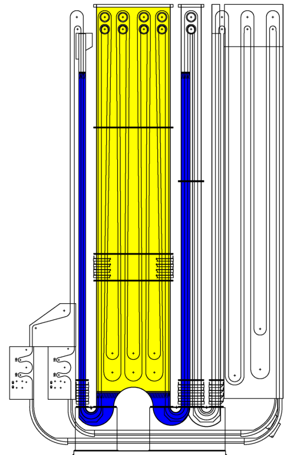
This diagram shows the feed and discharge center (bottom left), water (in blue), steam (in yellow), cooling area (right), and chains (two sets running through whole system).
